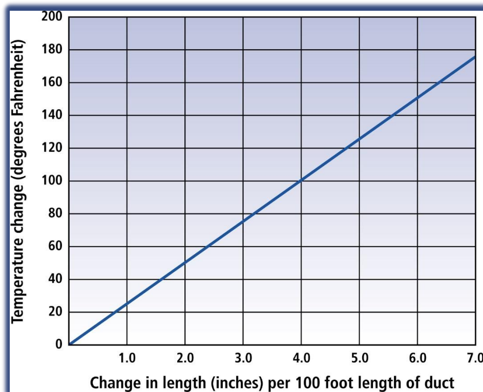
Expansion/Contraction Chart
